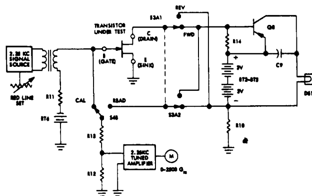
Figure 3-6. Field Effect Transistor Test
