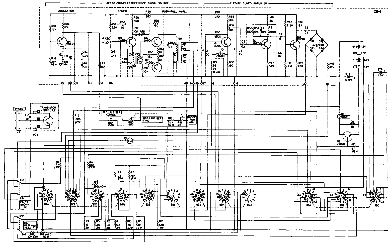
Figure 4-5. Model 219C In-Circuit Transistor Tester Schematic Diagram
