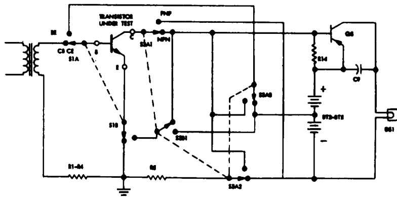
Figure 3-2. CE CB Short lost, NPN Transistor
