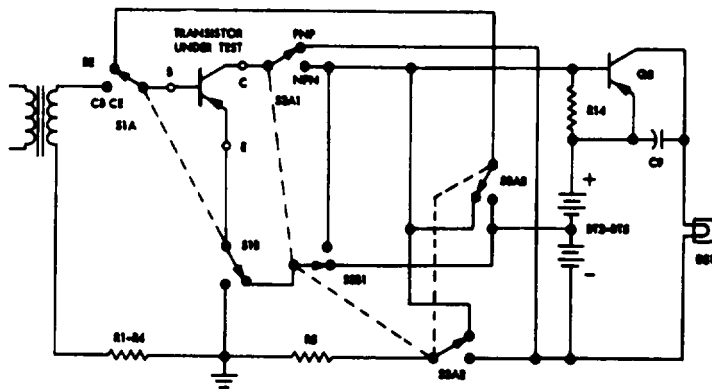
Figure 3-3. BE Short Test, PNP Transistor
