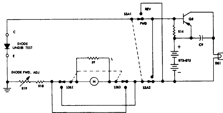
Figure 3-5. Diode Test
