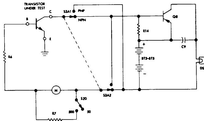
Figure 3-4. I_{\infty} Test
