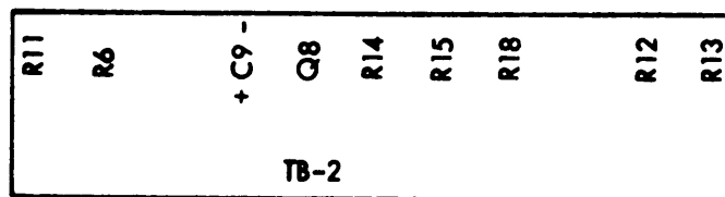
Figure 4-3. Component Location, Terminal Boards and Rear of Front Panel
